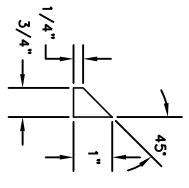
Front Angle 3/8" steel
